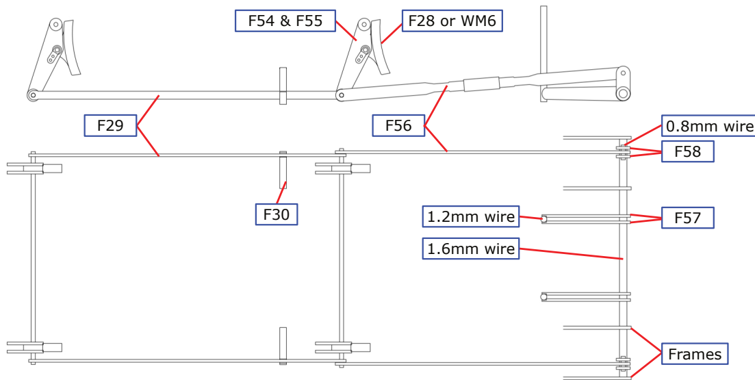
Fig 12. Brake Construction
