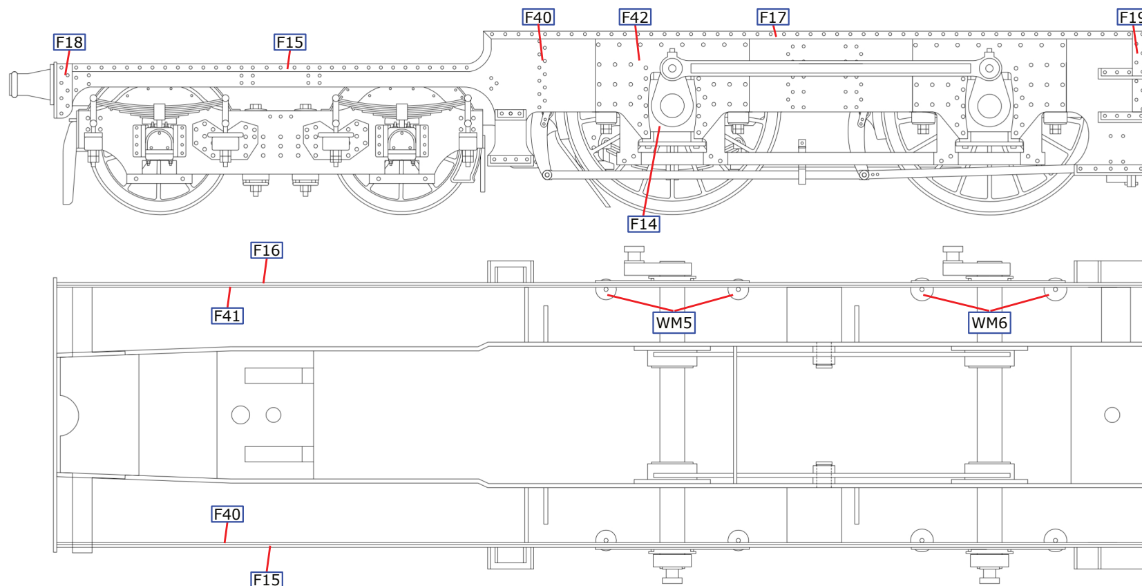
Fig 7. Frame Detailing
