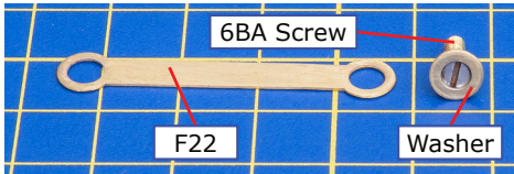
Fig 16. Drawbar
