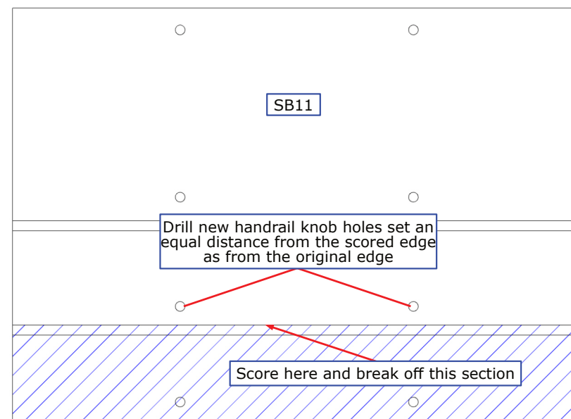
Fig 18. Boiler/Smokebox Wrapper Modification
