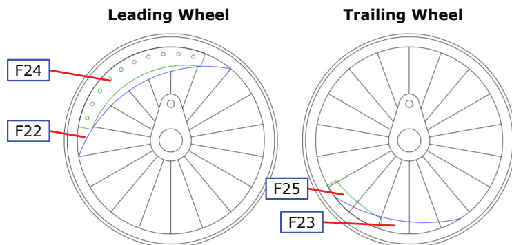
Fig 9. Wheel Balance Weights
