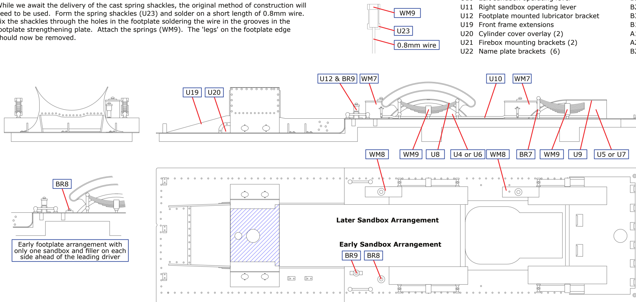
Fig 15. Footplate Construction
