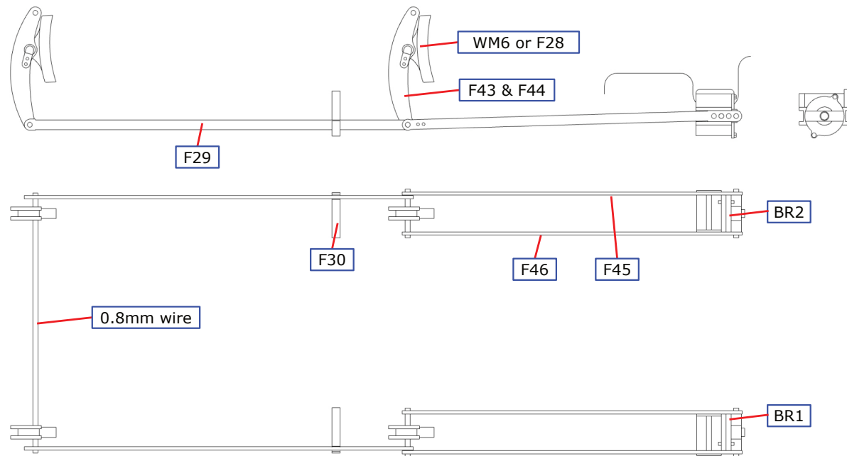
Fig 10. Bulldog Brake Construction
