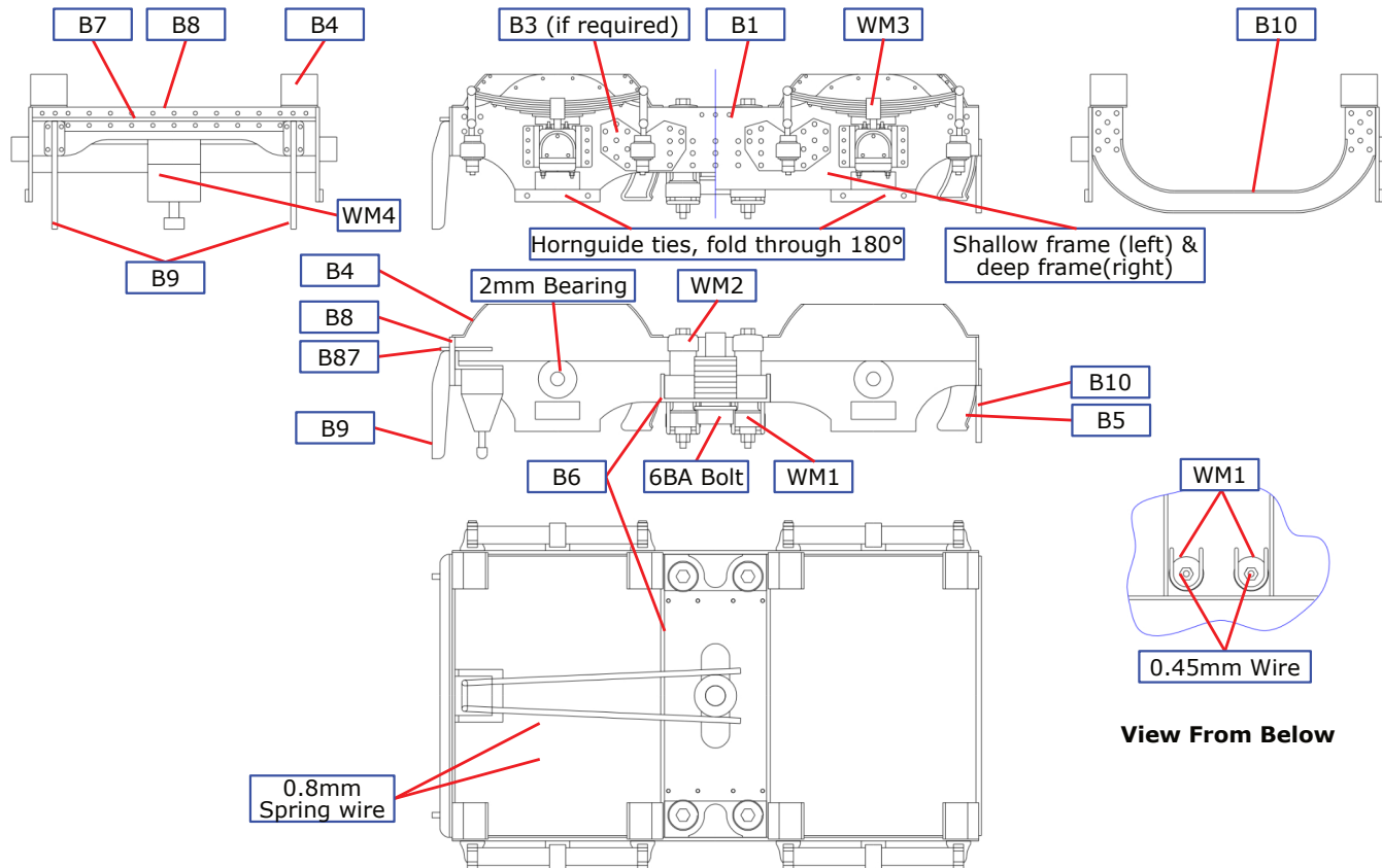
Fig 3. Bogie Construction
