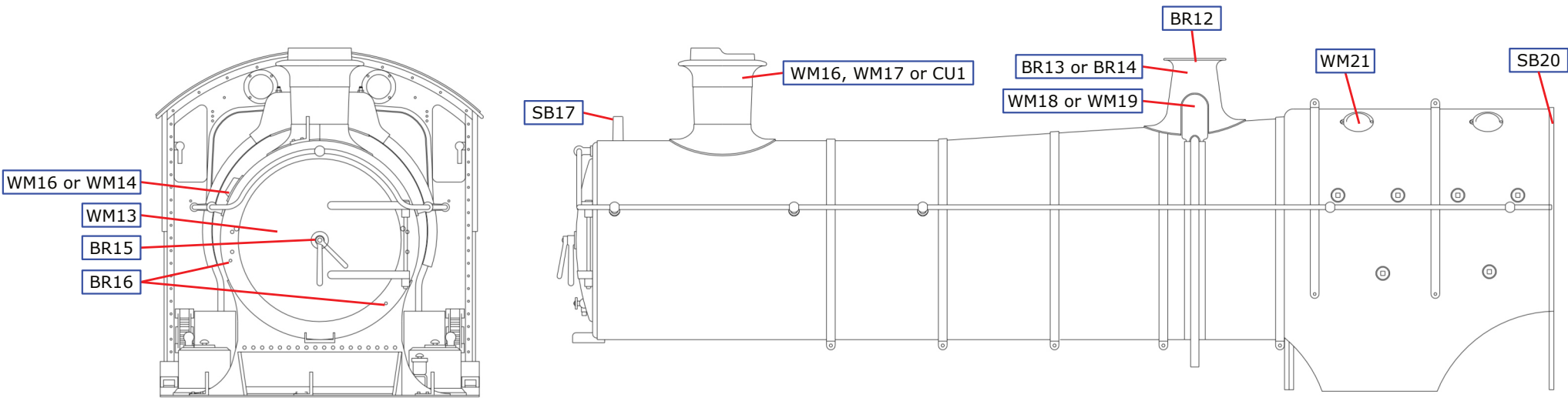
Fig 22. D3 Boiler Fittings
